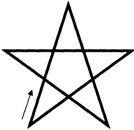
Figure B.I. Start at the lower left corner and trace the pentagram in the direction indicated until you come back to the starting point.
