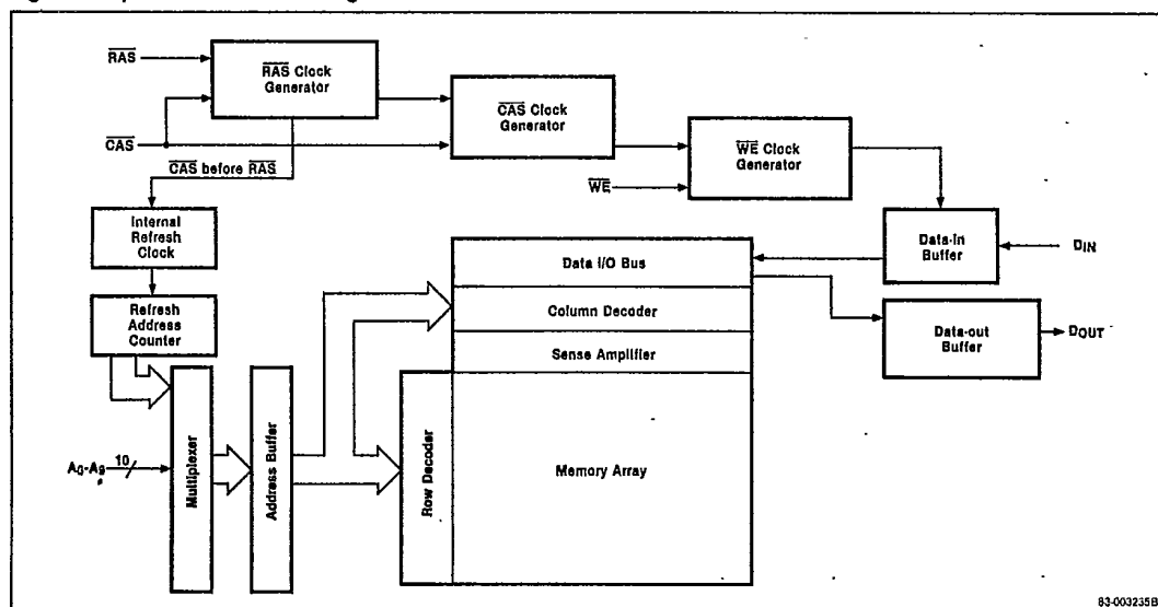
Figure 2. \mu PD421000 Block Diagram
