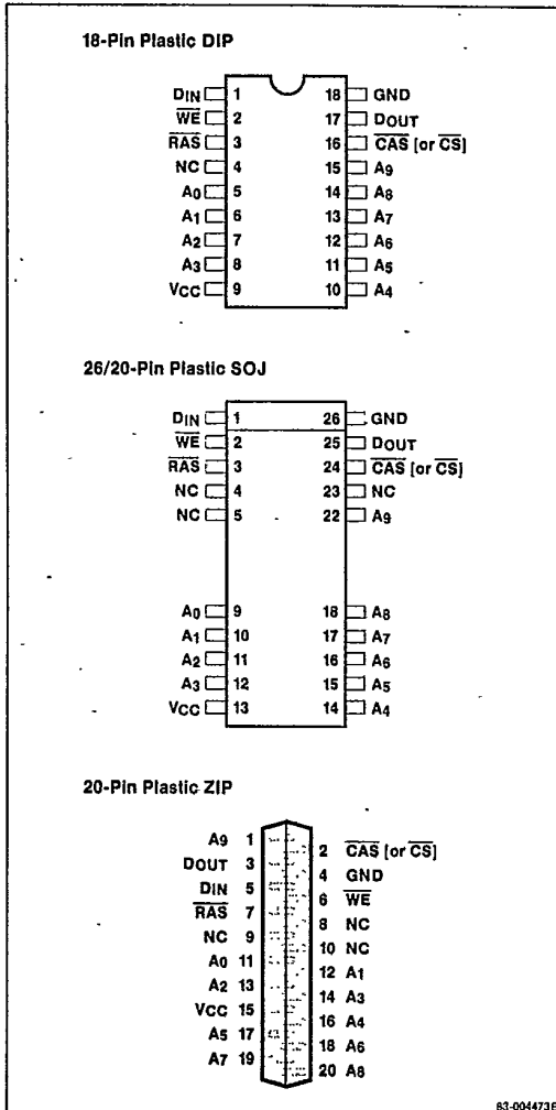
Figure 1. Pin Layouts
