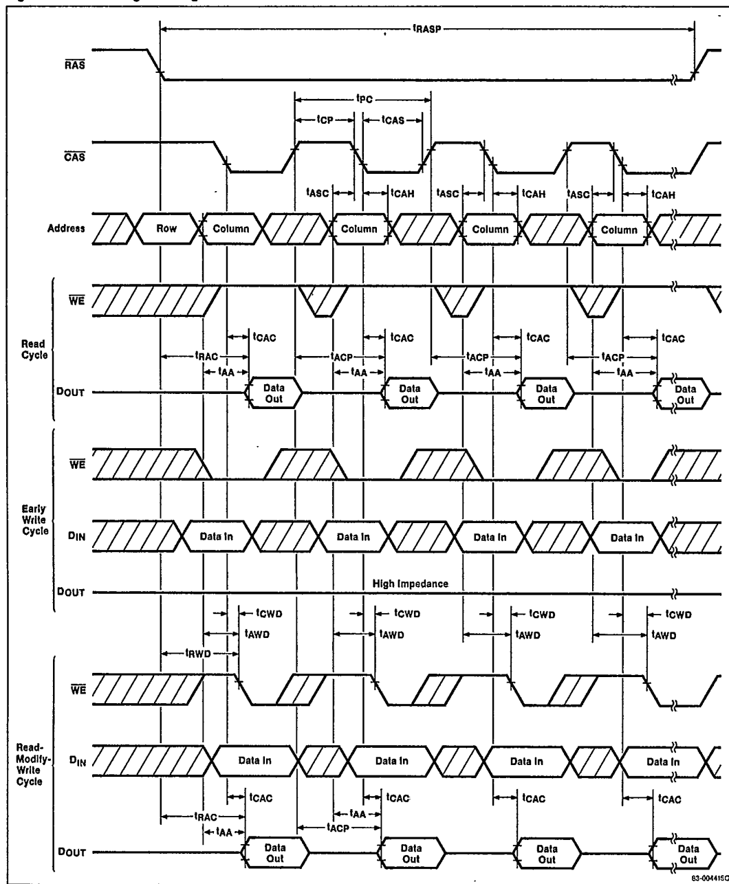
Figure 13. Fast-Page Timing
