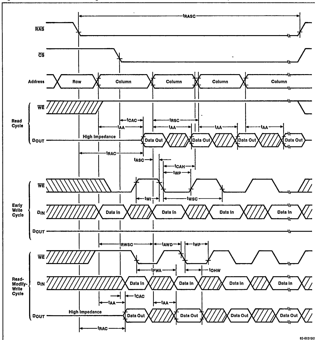
Figure 18. Static-Column Timing
