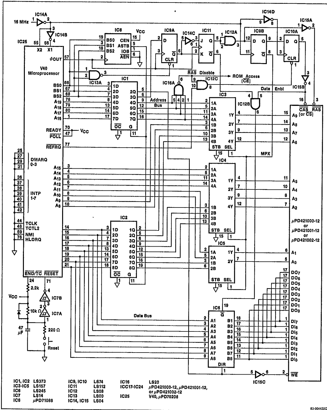
Figure 32. Composite Schematic
