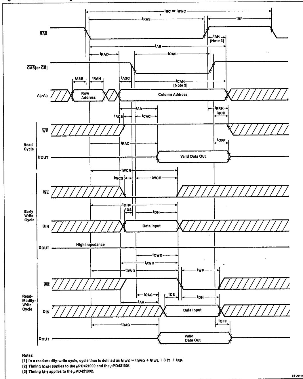
Figure 8. Access Timing
