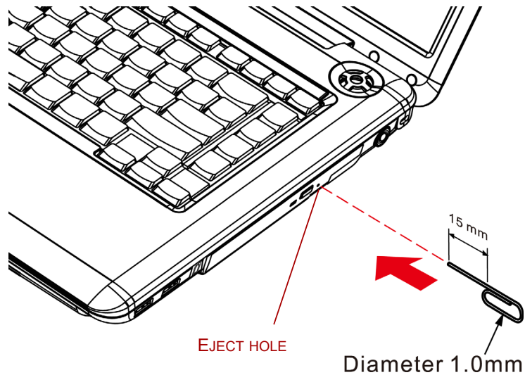
Figure 4-4 Manual release with the eject hole
