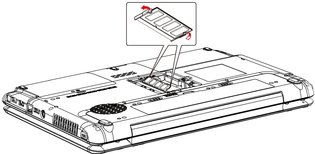
Figure 8-10 Removing the memory module
