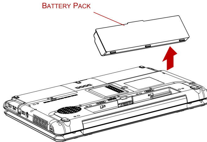
Figure 6-2 Removing the battery pack
