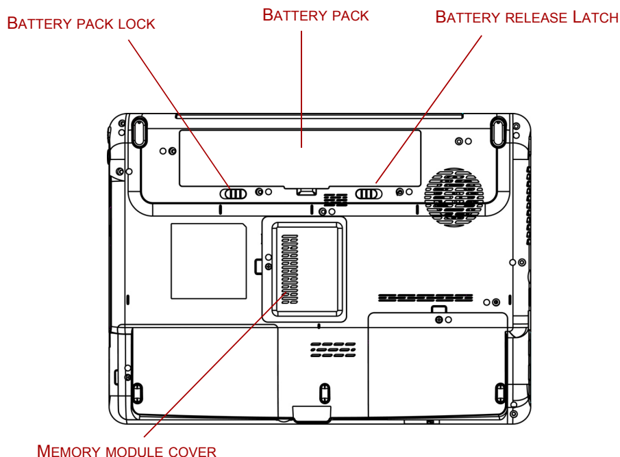
Figure 2-5 The underside of the computer
