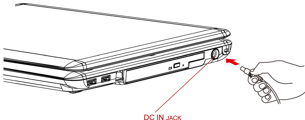
Figure 3-2 Connecting the adaptor to the computer
