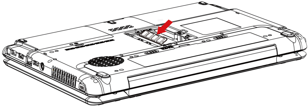
Figure 8-8 Inserting the memory module
