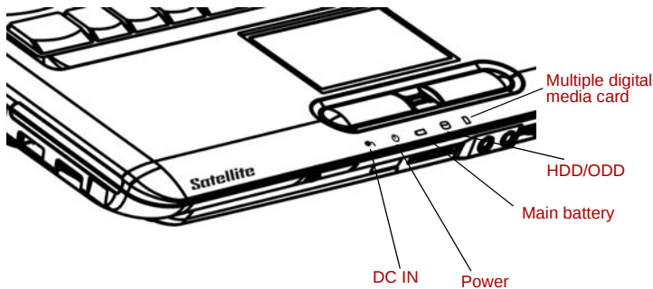
Figure 2-7 System indicators
