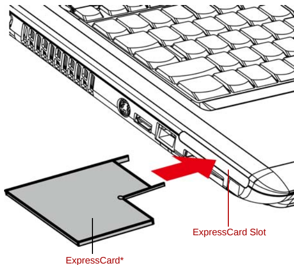
Figure 8-3 Inserting the ExpressCard
