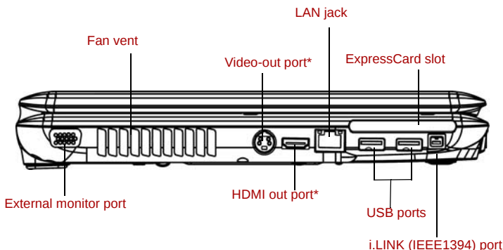
Figure 2-2 The left side of the computer
