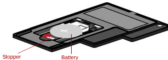
Figure 2-13 Inserting the batteries
