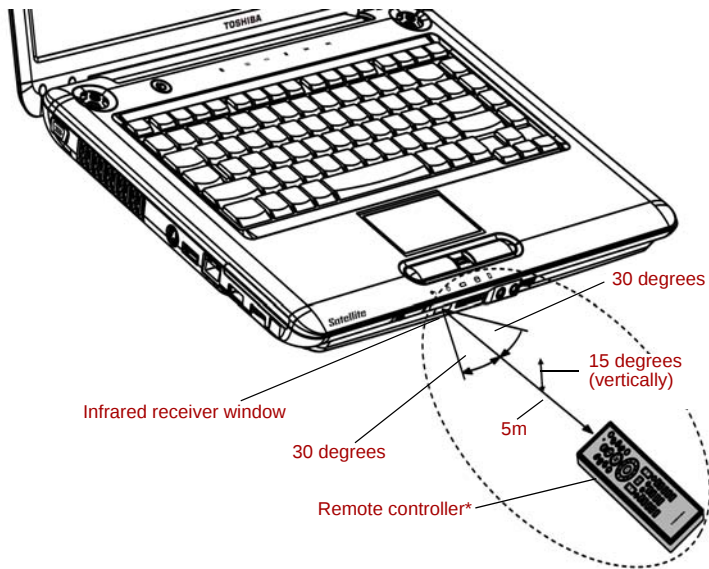
Figure 2-11 Operational range of the remote controller
