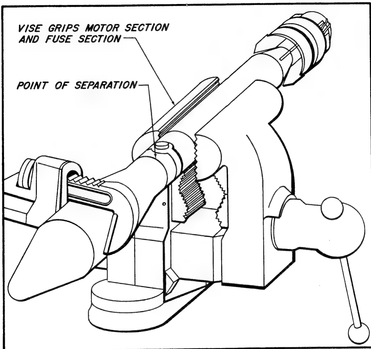
Fig. 52 — Removing Rocket Head
