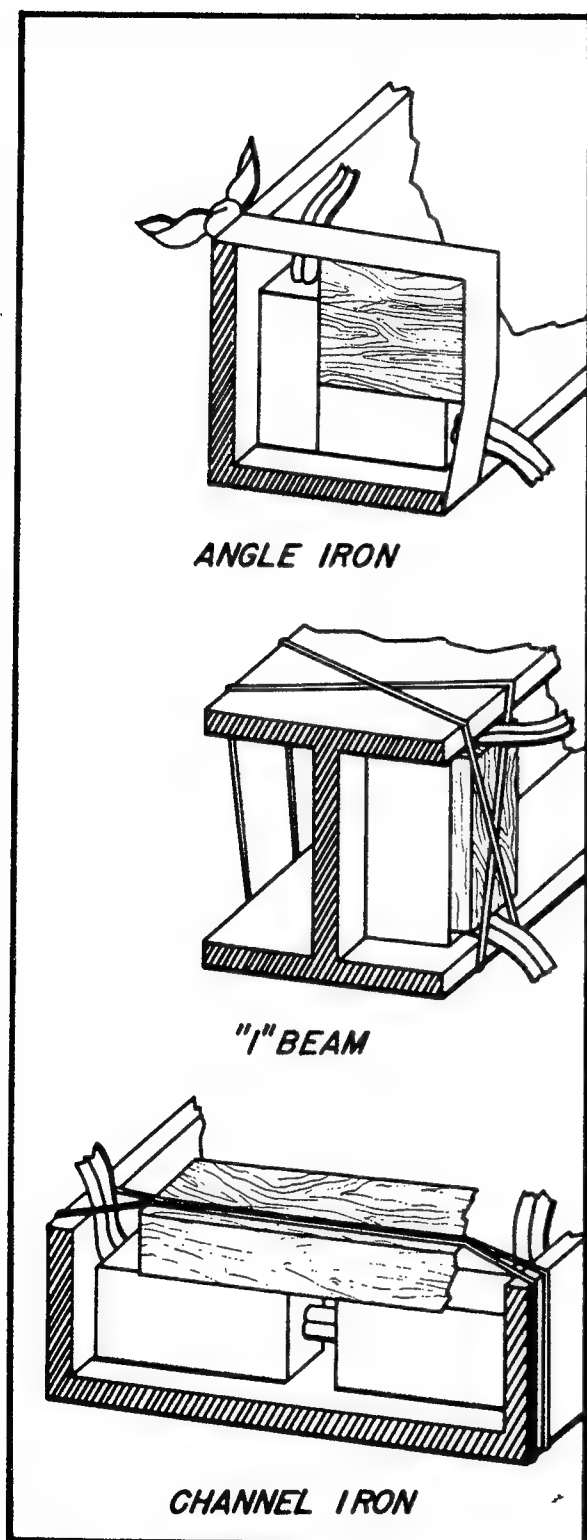
Fig. 28 — Standard Charge Placement
