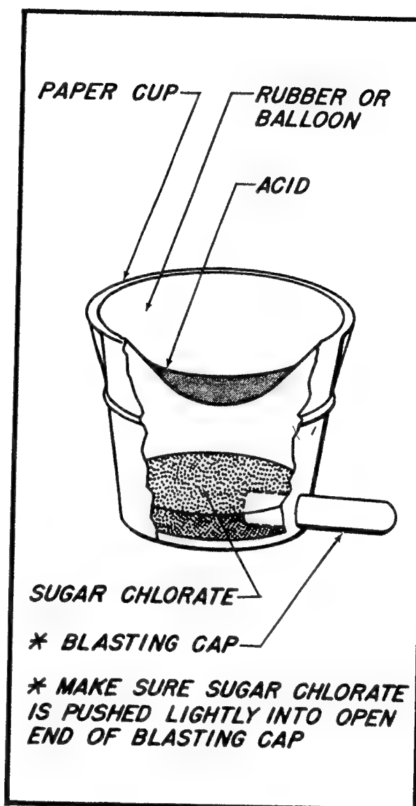
Fig. 16— Acid and Rubber Chemical Delay
