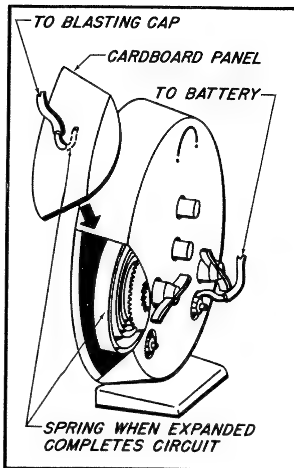
Fig. 11 — Seven Day Electric Delay
