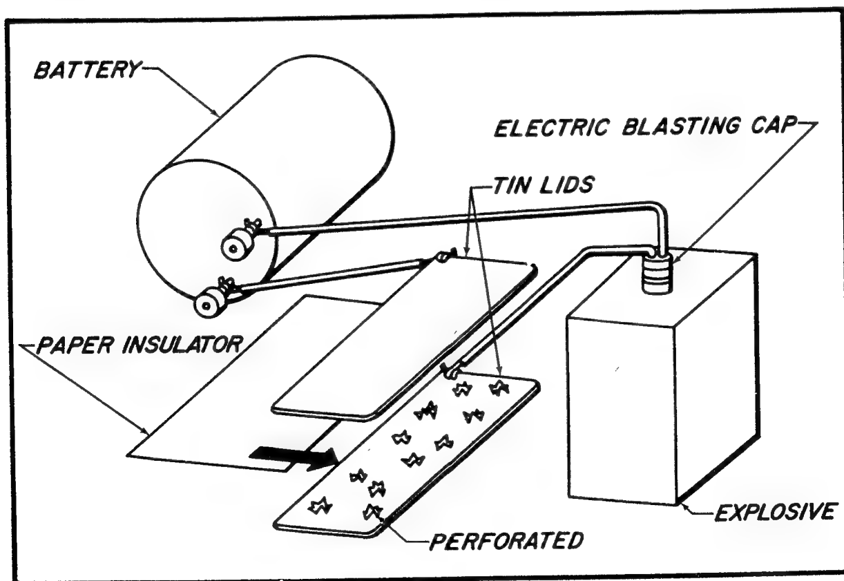
Fig. 6 — Electric Pressure Switch (Lids)
