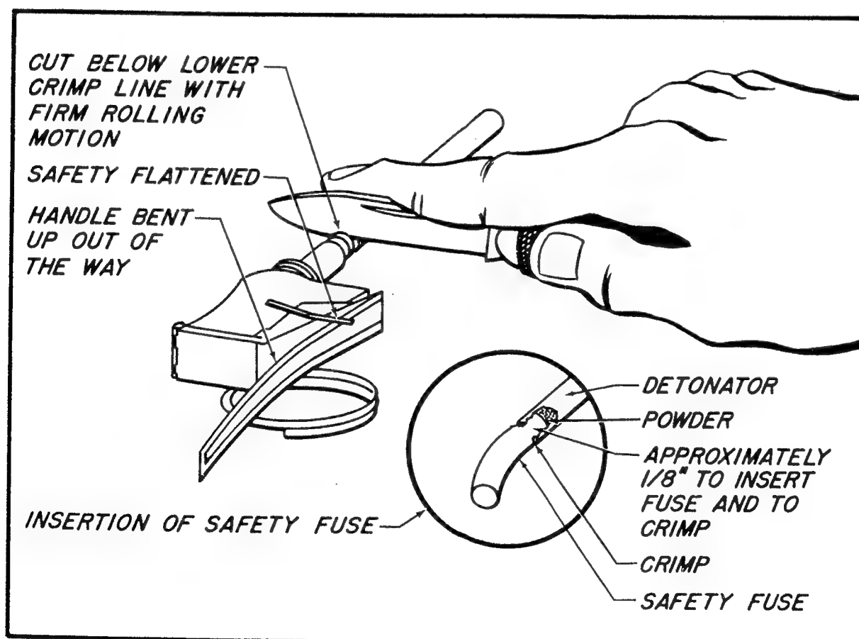
Fig. 22 — Removing Grenade Detonator
