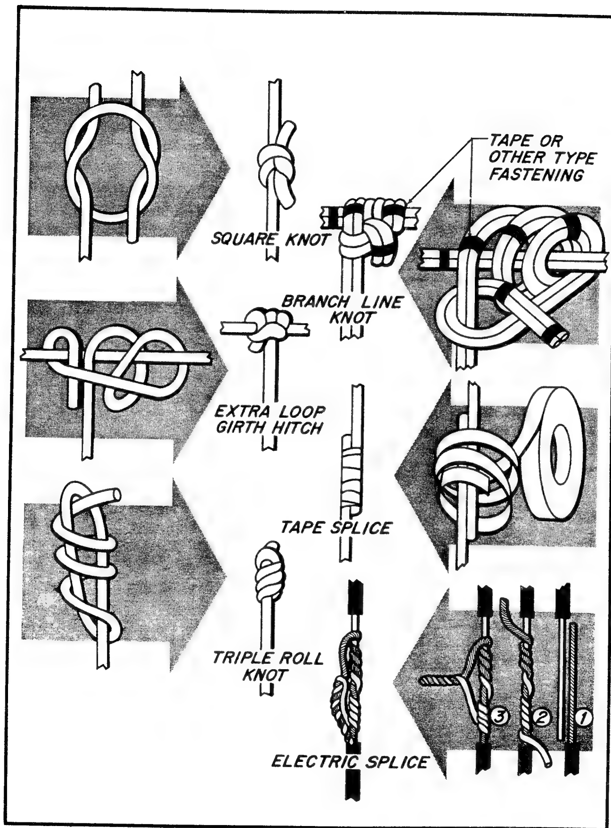
Fig. 5 — Splices and Knots
