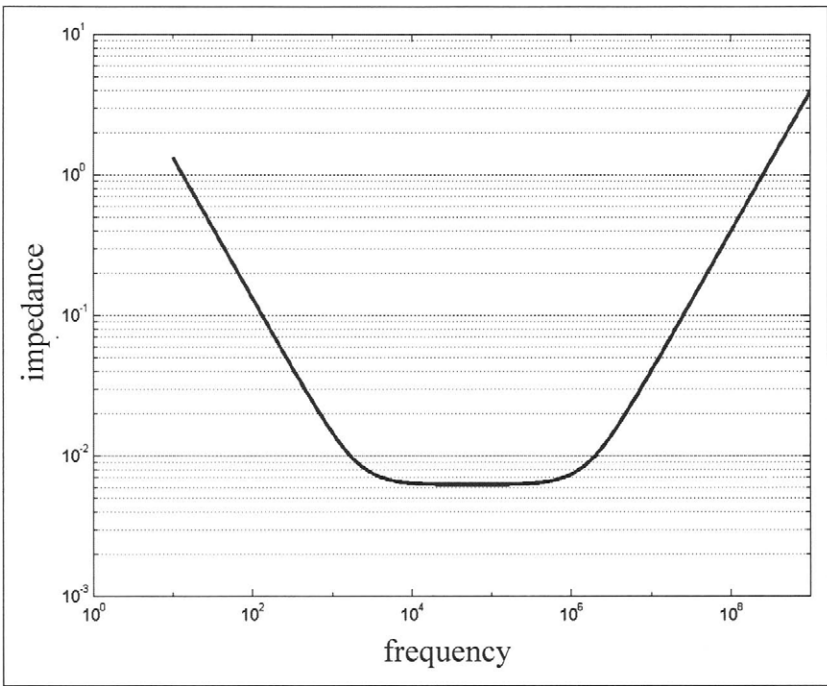
Figure 12.12 Frequency domain impedance of eight 1500μF capacitors.
