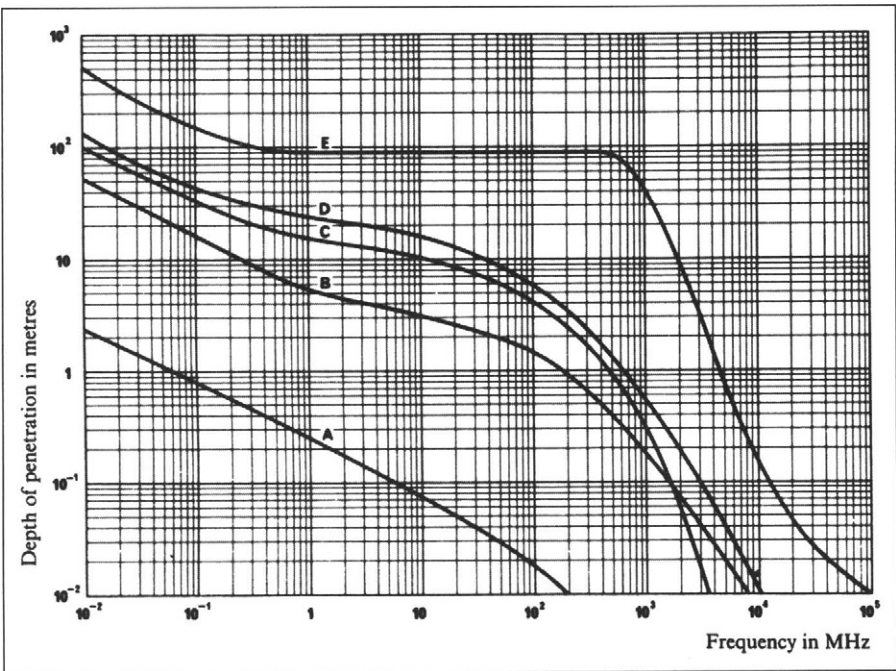
Figure 15.4 Penetration depth of waves into the Earth's surface: (A) sea water, (B) humid soil, (C) fresh water, (D) moderately dry soil, (E) very dry soil. Reproduced from Bolthas, L., Radio Wave Propagation , Boston: McGraw-Hill, 1987, p. 77, with permission of Kogan-Page, Ltd.
