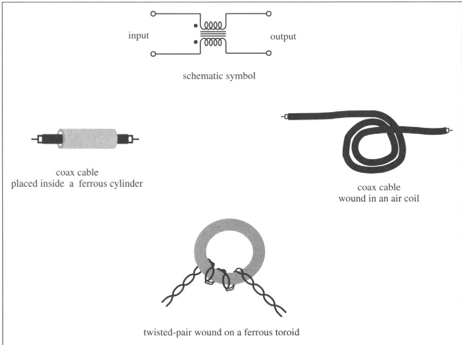
Figure 12.24 A common mode choke is constructed in the same manner as an inductor, except instead of winding a single wire, the common mode choke is wound using a transmission line.
