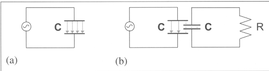
Figure 5.2 A) A capacitor creates a field that stores energy. B) Adding a second capacitor harnesses some of the storage field to transfer energy to the load resistor.
