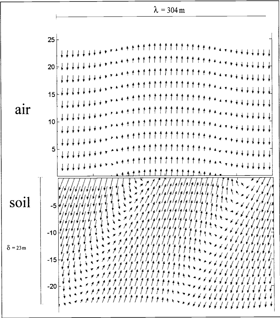
Figure 10.2 1 MHz surface wave on soil, traveling to the right. The arrows in the air represent about 10 times the magnitude of the arrows in the soil.
