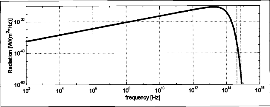
Figure 15.7 Thermal radiation spectrum of black body at 37°C (100°F). Note that the radiation in the visible band is about 23 orders of magnitude less than the peak radiation in the infrared.
