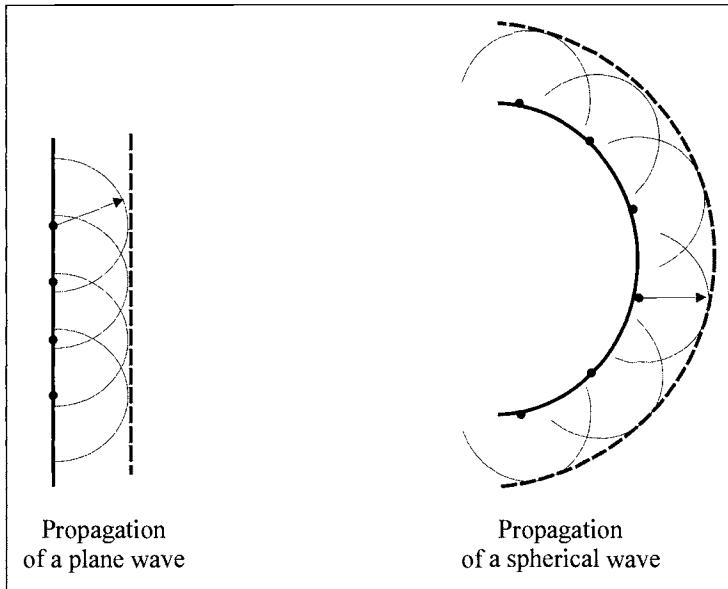
Figure 14.3 Demonstration of Huygens' principle. Each point of the initial wavefront creates its own spherical wavelet. The next wavefront (dotted line) is created from the outline of the individual wavelets.
