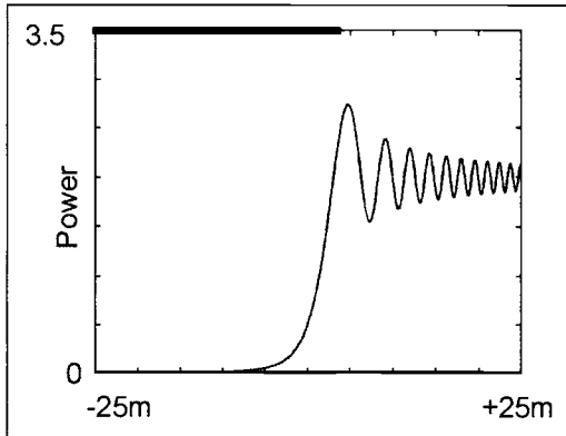
Figure 14.7 Simulated diffraction patterns at the edge of a long object, with incident radiation of 100MHz (3m wavelength). Pattern “measured” 10m from object. The figures graph the intensity of the radiation pattern.
