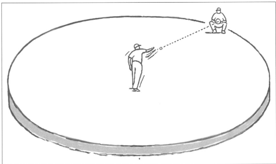
Figure 3.9 You throw a ball to your friend Bob. The platform is not spinning. The ball, therefore, travels straight to Bob.
