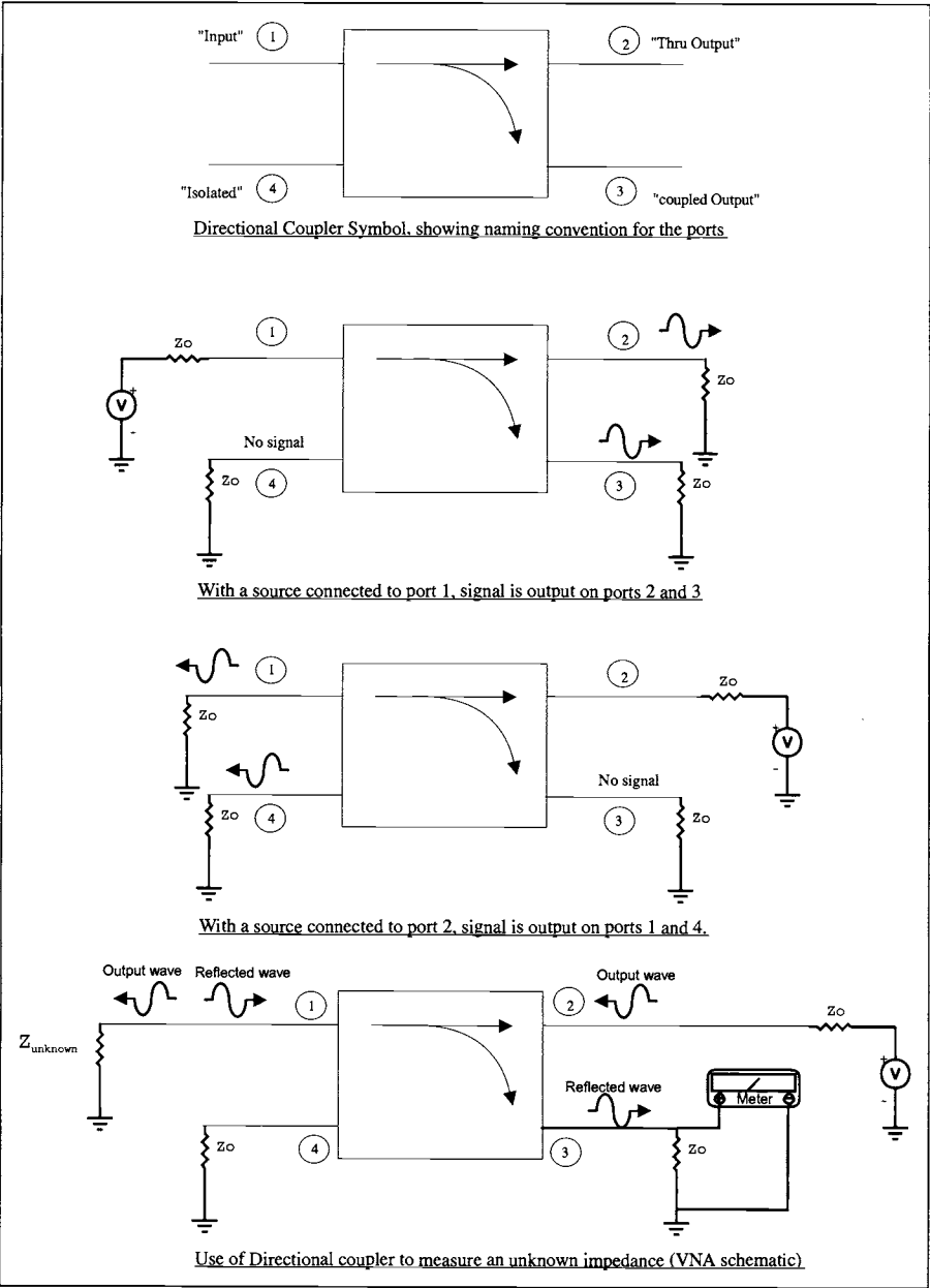
Figure 10.6 The directional coupler and examples of its use. Don't take the port names literally; the names are meaningful only when a signal is applied to port 1.
