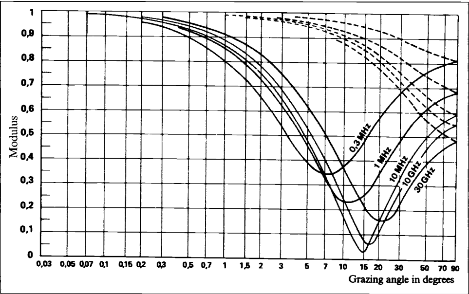
Figure 15.6 Soil reflectivity (moderately dry soil): dashed line represents horizontal polarization, solid line represents vertical polarization. Reproduced from Bolthas, L., Radio Wave Propagation , Boston: McGraw-Hill, 1987, p. 55, with permission of Kogan-Page, Ltd.
