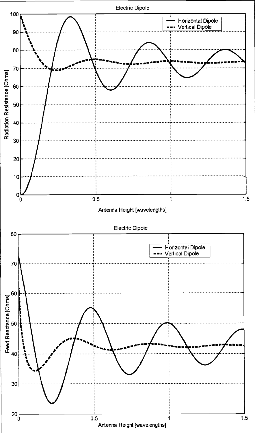
Figure 11.9 Feed/radiation resistance and feed capacitance for \lambda/2 electric dipoles versus height above ground.
