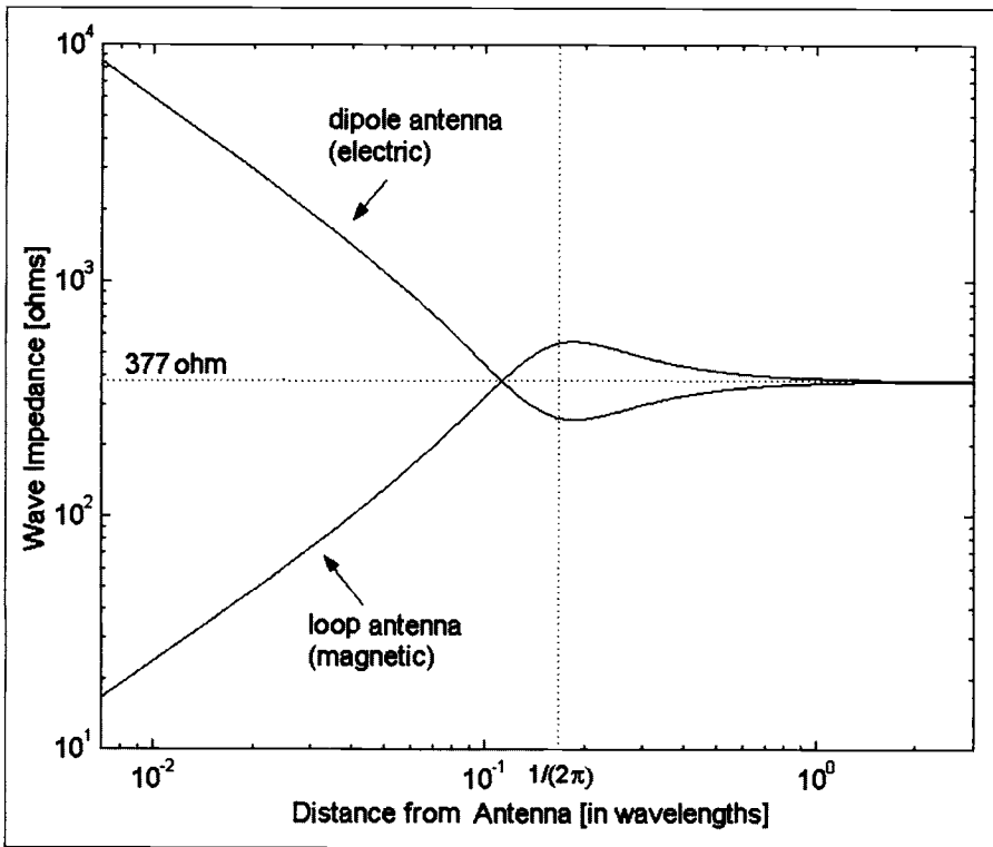
Figure 5.11 Compare the wave impedance as a function of distance given for a loop antenna (as in Figure 5.3A) and a dipole (as in Figure 5.3B). In the near field, the loop antenna field energy is mostly magnetic but the dipole antenna field energy is mostly electric. In the far field, the energy partitioning is the same for both antenna types.
