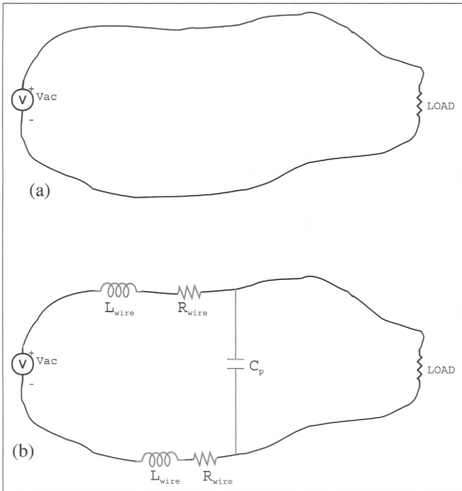
Figure 7.7 A) A simple circuit consisting of a voltage source connected to a load resistor. B) The hidden schematic for the wires includes resistance ( R_{\text{wire}} ), inductance ( L_{\text{wire}} ), and parasitic capacitance ( C_p ).
