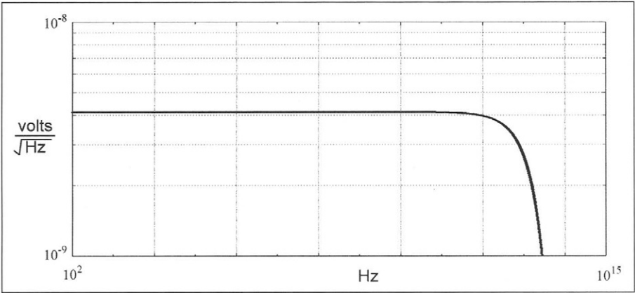
Figure 15.10 Voltage noise spectrum of a 1 kohm resistor at 37°C (100°F). The noise is white up into the infrared.
