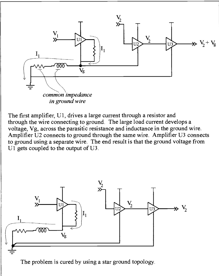
Figure 12.9 Demonstration of common impedance coupling, ground bounce, and star grounding.
