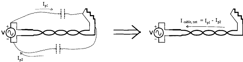
Figure 12.23 Common mode currents arise due to asymmetries in circuits. The circuit asymmetries give rise to asymmetric parasitic paths, leaving a net current on the cable. The net common mode current acts as an efficient antenna.
