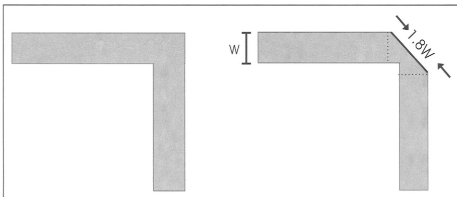
Figure 12.13 90 degree turns on PCB transmission lines. The uncompensated 90 degree turn (left) is satisfactory below 1 GHz. For higher frequencies, it may be necessary to compensate for the bend by chamfering the corner (right).
