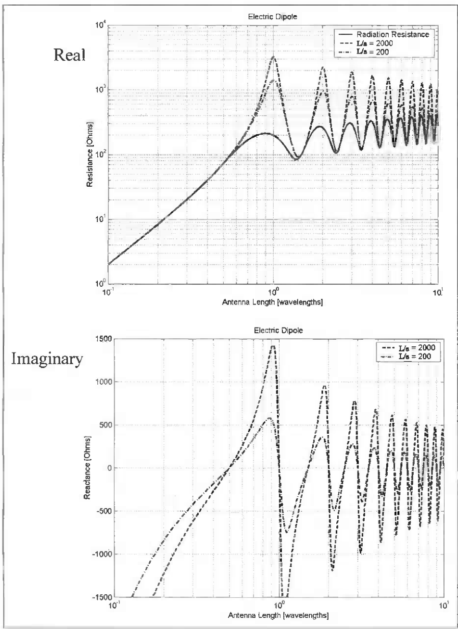
Figure 11.5 Feed (input terminal) impedance of an electric dipole as a function of antenna length. For reference, the radiation resistance is shown as a solid line. At a half wavelength, the feed impedance is equal to the radiation resistance. At a wavelength, the feed impedance has a large inductive reactance and the feed resistance is substantially larger than the radiation resistance. Feed impedance is also highly dependent on the wire radius of the antenna. The plots show feed resistance for two different ratios of length to radius.
