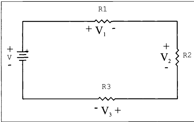
Figure 1.2 A simple circuit demonstrating Kirchhoff's voltage law ( V = V_1 + V_2 + V_3 ).
