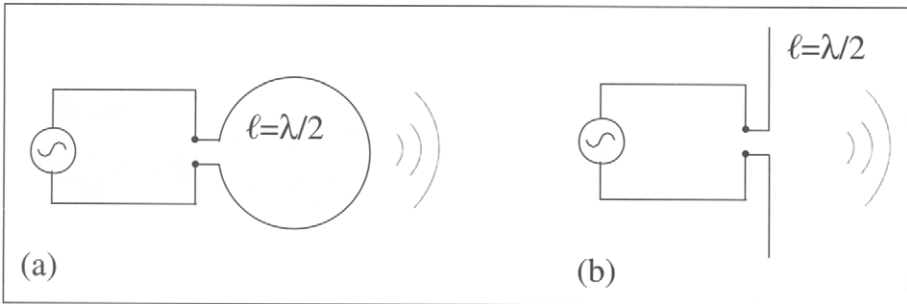
Figure 5.3 The two most basic antennas are: A) a loop antenna whose circumference is equal to the source wavelength divided by two, and B) a dipole antenna whose length is equal to the source wavelength divided by two.
