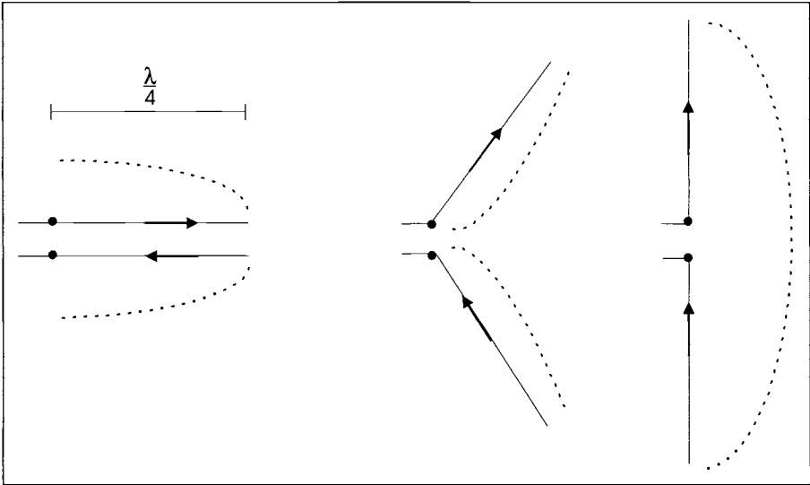
Figure 11.1 A dipole antenna can be created by pulling apart an open-circuit transmission line. The arrows denote the direction of current, and the dotted lines indicate current magnitude.
