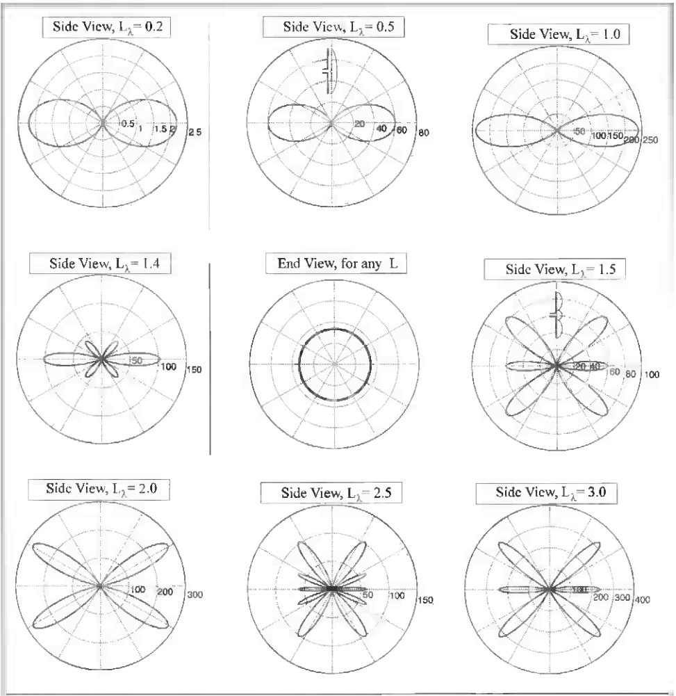
Figure 11.7 Radiation patterns for electric dipoles of various electrical lengths. In each case, the antenna is driven with 1 A. The current on the antenna is shown for lengths of 1/2 and 3/2 . The center plot shows the end-view pattern for all lengths.
