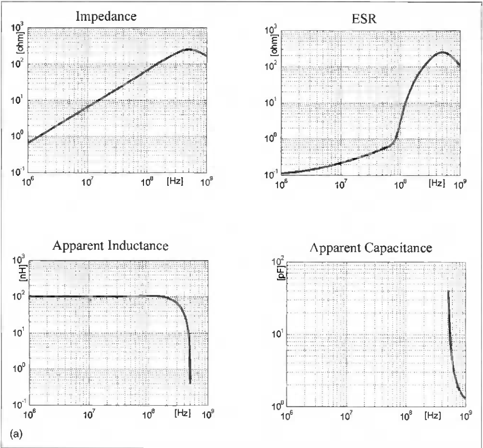
Figure 7.6 A) Frequency response of a ferrite-core, 100 nH surface-mount inductor ( C_p = 1 pF; R_{DC} = 0.26 ohm). Above about 80 MHz, the ESR increases dramatically due to ferrite losses in the core. The self-resonant frequency occurs at about 500 MHz. Above the self-resonant frequency, the device acts like a \sim 1 pF capacitor.
