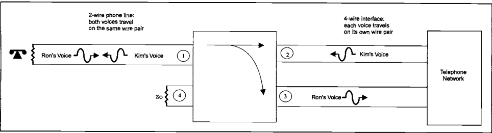
Figure 10.8 The telephone line directional coupler (a.k.a., 2-wire/ 4-wire hybrid).
