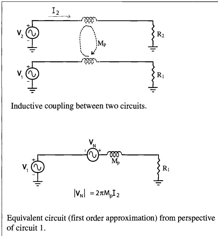
Figure 12.4 Magnetic field (inductive) coupling and equivalent circuit.
