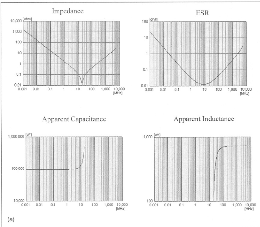
Figure 7.4 A) Frequency response of a 0.1 \mu\text{F} surface-mount, size 0805 (0.08" \times 0.05") capacitor ( L_{\text{lead}} = 0.73 \text{ nH} ). B) Frequency response of a 0.015 \mu\text{F} surface-mount, size 0805 (0.08" \times 0.05") capacitor ( L_{\text{lead}} = 0.88 \text{ nH} ). Above the self-resonant frequency (SRF) of \sim 40 \text{ MHz} , the device acts like a 0.88 nH inductor. C) Frequency response of a 0.001 \mu\text{F} surface-mount, size 0805 (0.08" \times 0.05") capacitor ( L_{\text{lead}} = 0.77 \text{ nH} ). Above the self-resonant frequency (SRF) of \sim 200 \text{ MHz} , the device acts like a 0.77 nH inductor. Plots were created with muRata's MCSIL software ( http://www.murata.com/ ).
