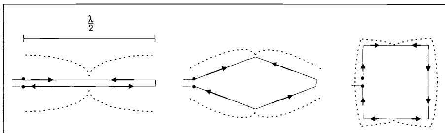
Figure 11.2 A loop antenna can be created by pulling apart a short-circuit transmission line. The arrows denote the direction of current, and the dotted lines indicate current magnitude.
