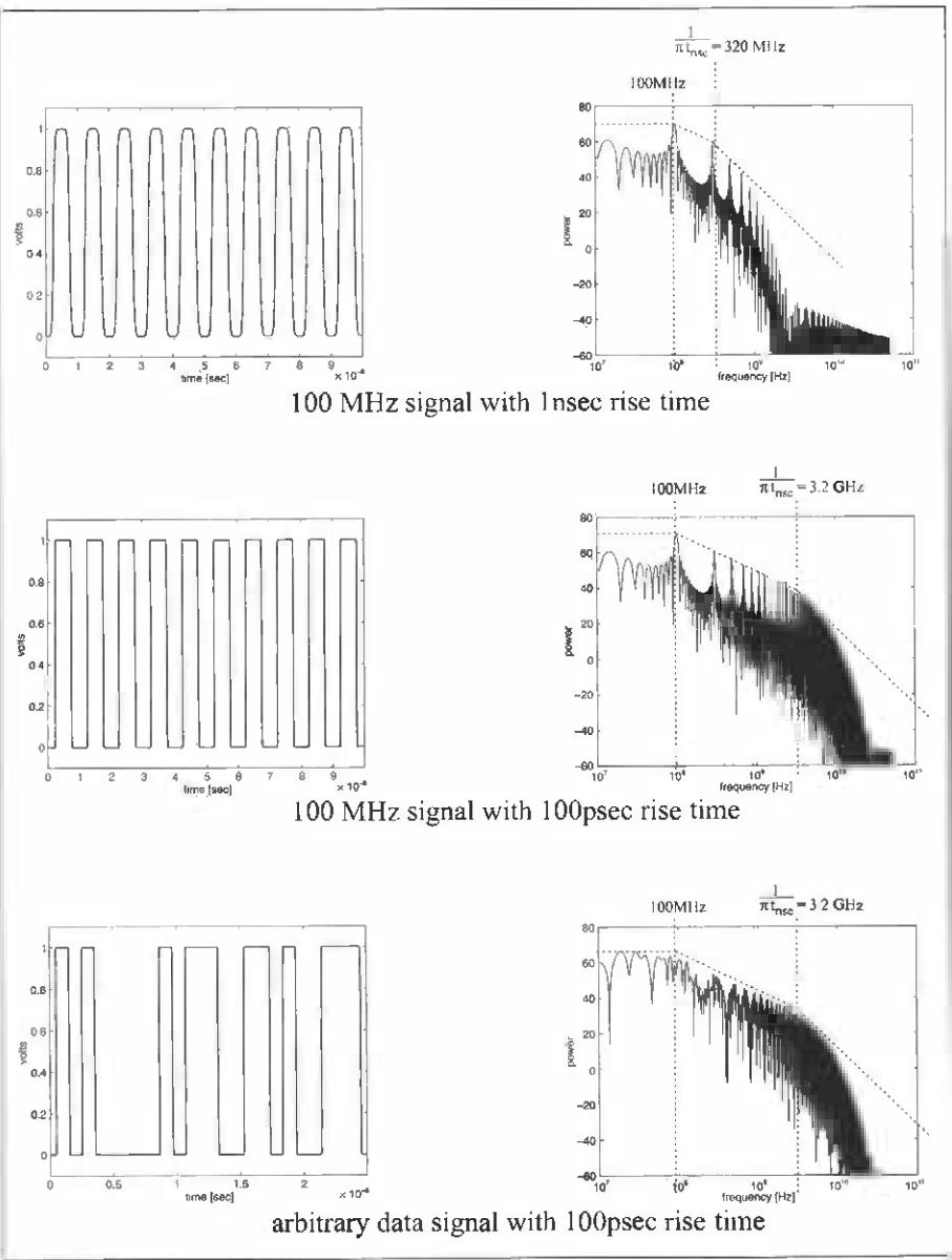
Figure 12.2 Some digital signals and their frequency spectra. The frequency spikes occur at the clock frequency and odd harmonics of the clock frequency. The rise time determines how fast the harmonics decay, and thus determines the overall shape of the curve.
