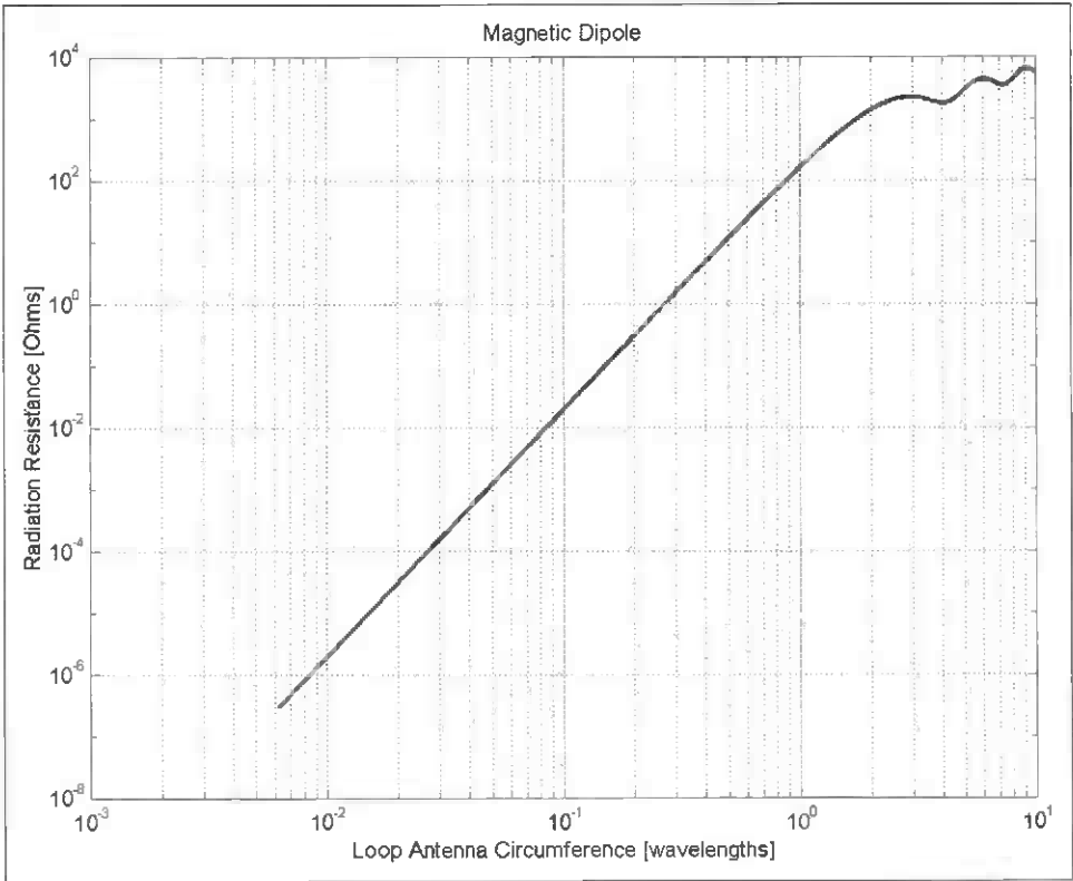
Figure 11.4 Radiation resistance versus magnetic dipole circumference. Below a wavelength, the radiation resistance is proportional to C_\lambda^4 . Power radiated can be determined using P = I^2 \times R_{rad} . This plot assumes a constant current around the loop, and loses accuracy above a half wavelength. However, the general behavior of large loop antennas is similar.
