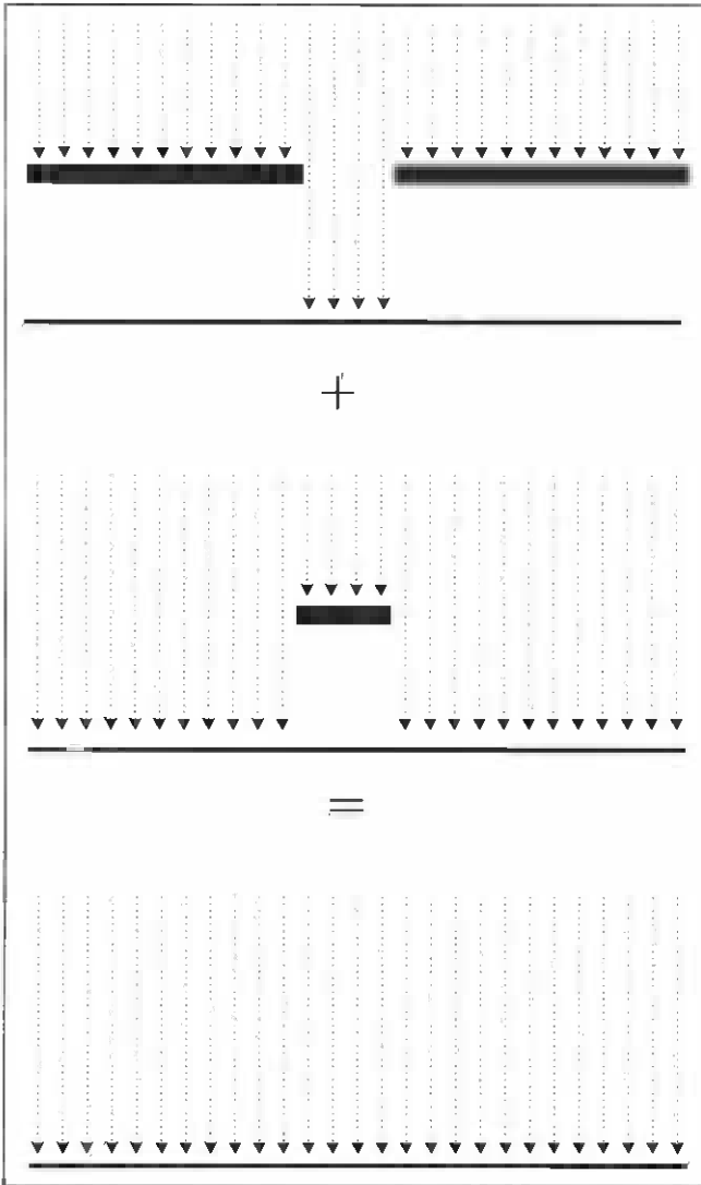
Figure 14.4 Illustration of Babinet's principle. The sum of the light patterns of an aperture and an object of equal size and shape is equal to the pattern without any barriers.
