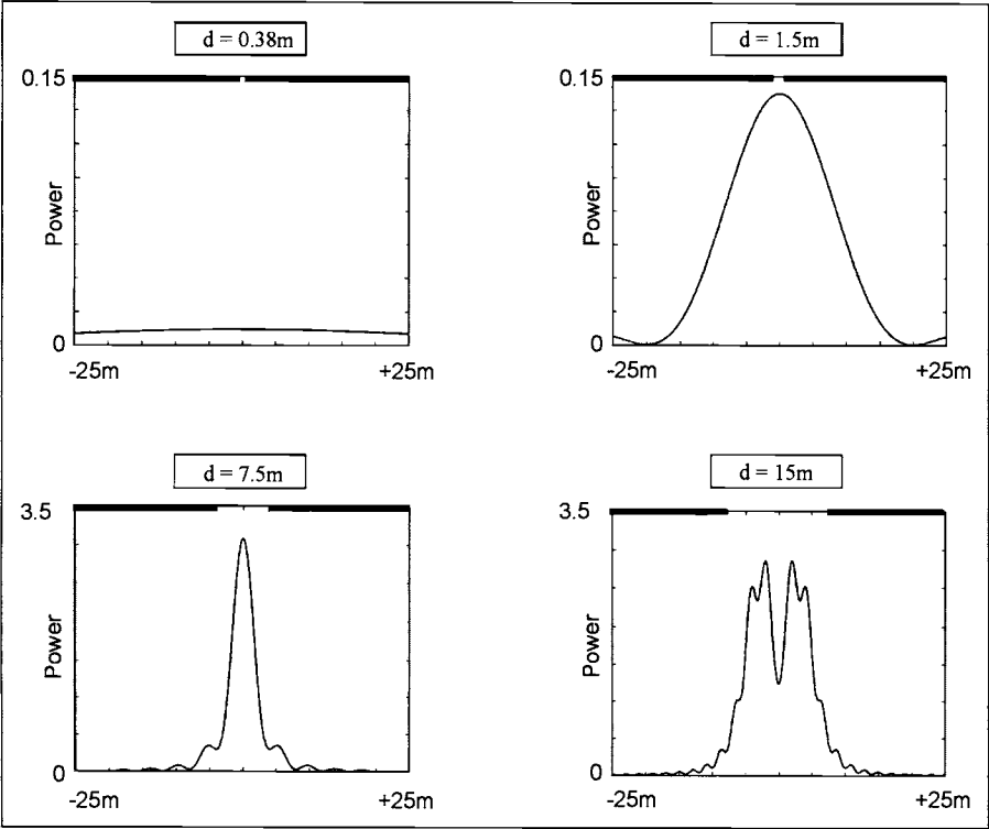
Figure 14.5 Simulated diffraction patterns for apertures of various widths, with incident radiation of 100MHz (3 m wavelength). Patterns “measured” 10 m from aperture. The figures graph the intensity of the radiation pattern.
