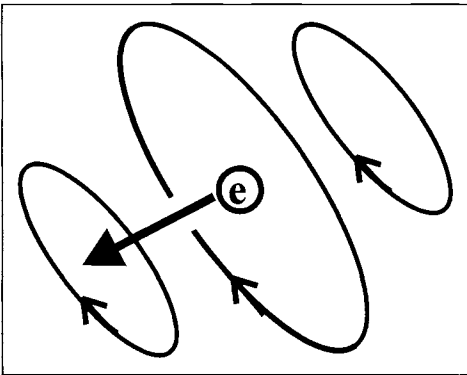
Figure 3.2 Magnetic field lines surround a moving electron.
