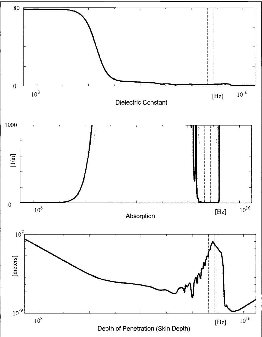
Figure 15.2 Electrical properties of water as a function of frequency. Dotted lines mark the visible region of the spectrum. Data compiled from D.J. Segelstein, "The complex refractive index of water," M.S. Thesis, University of Missouri-Kansas City, (1981). Data available online at http://omlc.ogi.edu/spectra/index/html .
