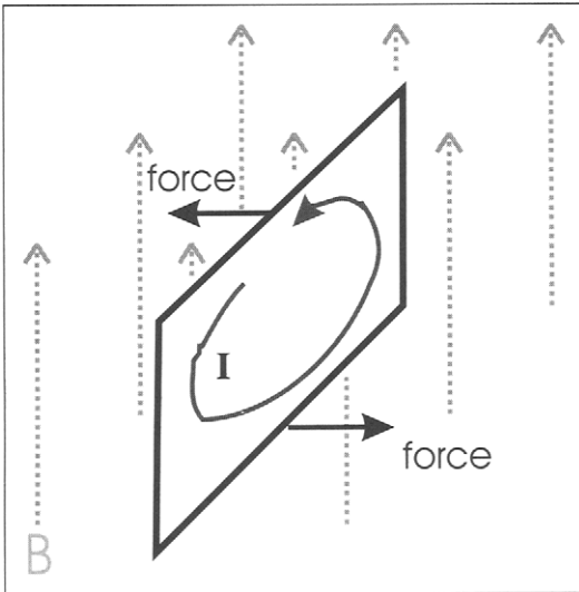
Figure 3.15 A current-carrying loop experiences a torque (rotational force) causing it to line up with an applied magnetic field.
