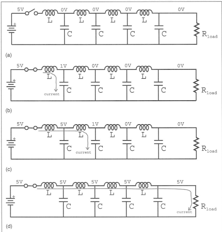
Figure 8.2 A conceptual demonstration of transmission line delay and characteristic impedance. A battery is connected to a resistor through a transmission line, which is represented by a series of L-C stages. A) The switch is open. No current flows and the voltage of the transmission line is zero everywhere. I = 0 . B) The switch is closed. Current flows and starts charging the first L-C stage. I = V_{\text{battery}}/Z_o , where Z_o = \sqrt{L/C} . C) The battery has charged the first stage and is now charging the second stage. I = V_{\text{battery}}/Z_o . D) The battery has charged the entire transmission line, and now current flows through the load resistor. I = V_{\text{battery}}/R_{\text{load}} .
