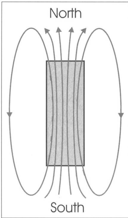
Figure 3.6 Magnetic field lines surrounding a bar magnet.
