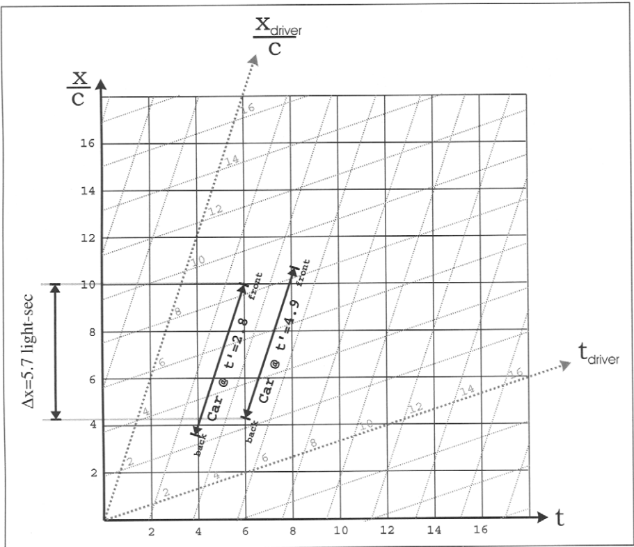
Figure 6.4 Lorentz contraction. You measure the moving car at time t = 6 secs by taking a photograph. In the driver's frame, the parts of the car are photographed at different points in time. The front of the car is photographed at t' = 2.8 sec and the back of the car is photographed at t' = 4.9 sec. The rest of the car is photographed at intermediate times. This effect causes the car to appear shorter in your frame.
