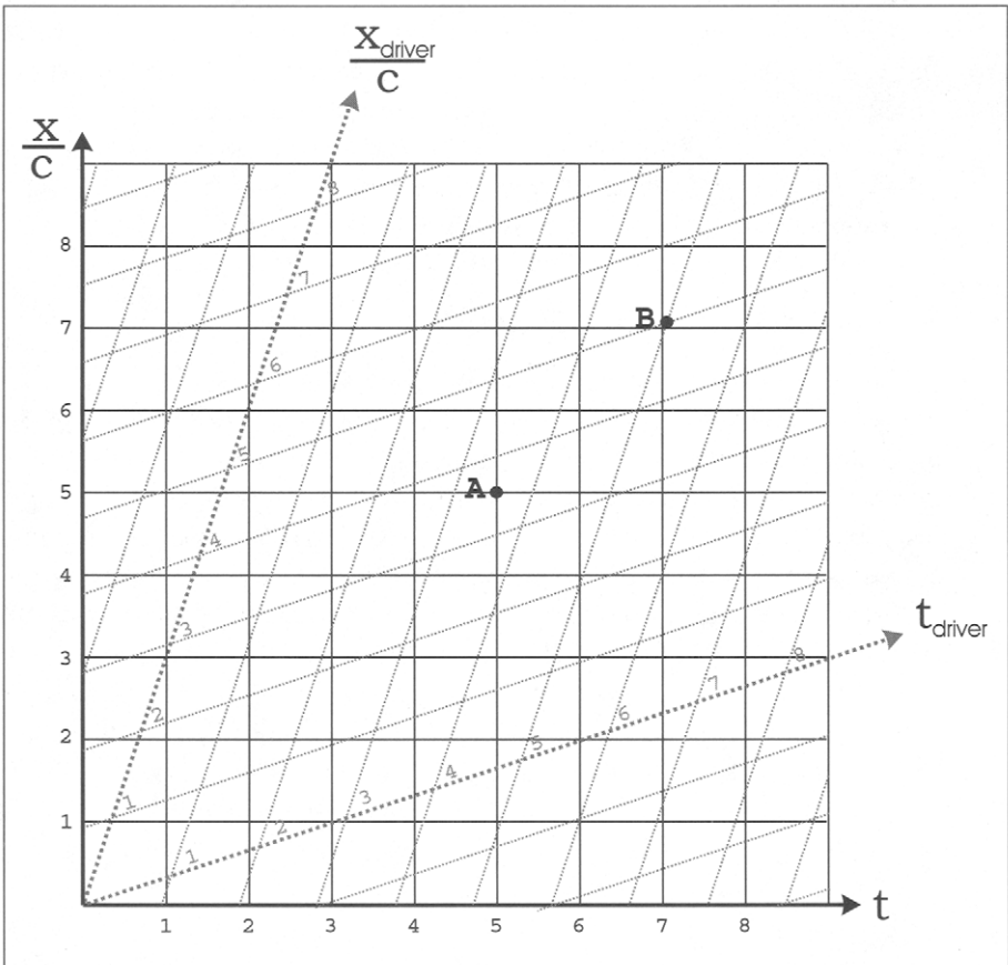
Figure 6.1 Space-time map. Axes of the reference observer (you) are shown in black. Axes of the other observer (driver) are shown in gray. The driver's time axis has a slope, v/c . The driver's distance axis has a slope c/v . Both of the driver's axes are also stretched by a factor \gamma \cdot \sqrt{1 + (v/c)^2} . Event A occurs at t = 5 sec, x = 5 light-secs, in your frame and at t' = 3.5 sec, x' = 3.5 light-secs, in the driver's frame. Event B occurs at t = 7.1 sec, x = 7.1 light-secs, in your frame and at t' = 5 sec, x' = 5 light-secs, in the driver's frame.
