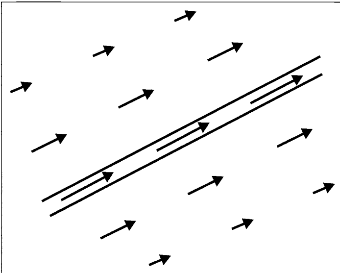
Figure 3.16 A plot of the magnetic vector potential surrounding a current-carrying wire.
