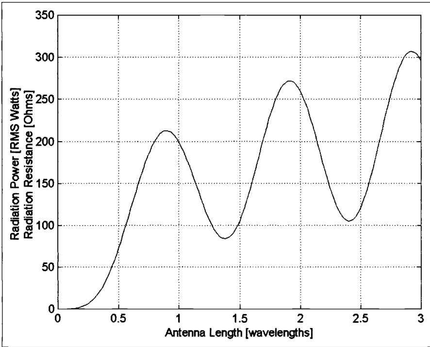
Figure 5.10 The root-mean-square radiation power versus electrical length for a dipole antenna driven by 1 ampRMS of current. The radiation resistance follows the same curve. At one-half wavelength the resistance is 73 ohms.
