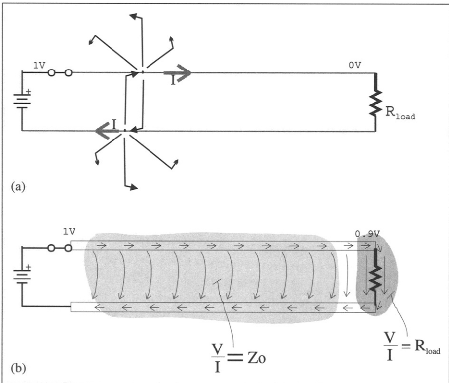
Figure 10.3 A) A pulse traveling down a transmission line.* The direction of current is shown by the gray arrows. The top charge moves to the right; the bottom charge moves to the left. The black arrows show the electric field caused by each moving charge. As you can see, the fields of each charge reinforce the movement. (The charges are assumed to be positive [+] for simplicity.) The charges carry this pulse of energy to the right. B) The electric field lines after steady state has been established. Inside the wire, the electric field lines point in the direction of the current. The wave impedance between the wires of the transmission line is equal to the characteristic impedance of the line. The wave impedance in the neighborhood of the load resistor is equal to the resistance of the load. To see an “end-on” view of the field surrounding the load, refer to Figure 2.15.
