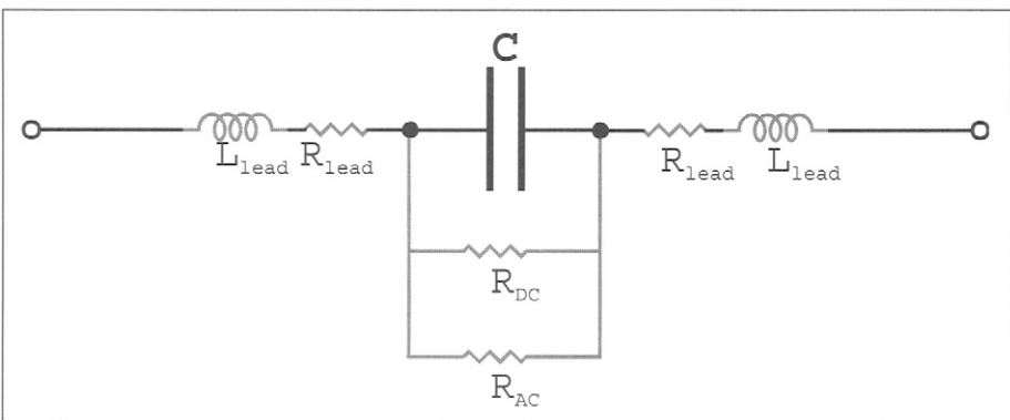
Figure 7.3 The hidden schematic of a real-world capacitor includes lead inductance ( L_{\text{lead}} ), lead resistance ( R_{\text{lead}} ), dielectric leakage ( R_{\text{DC}} ), and dielectric “frictional” loss ( R_{\text{AC}} ). The resistances are often combined and called Equivalent Series Resistance (ESR). Dielectric losses (and hence ESR) are typically frequency dependent.
