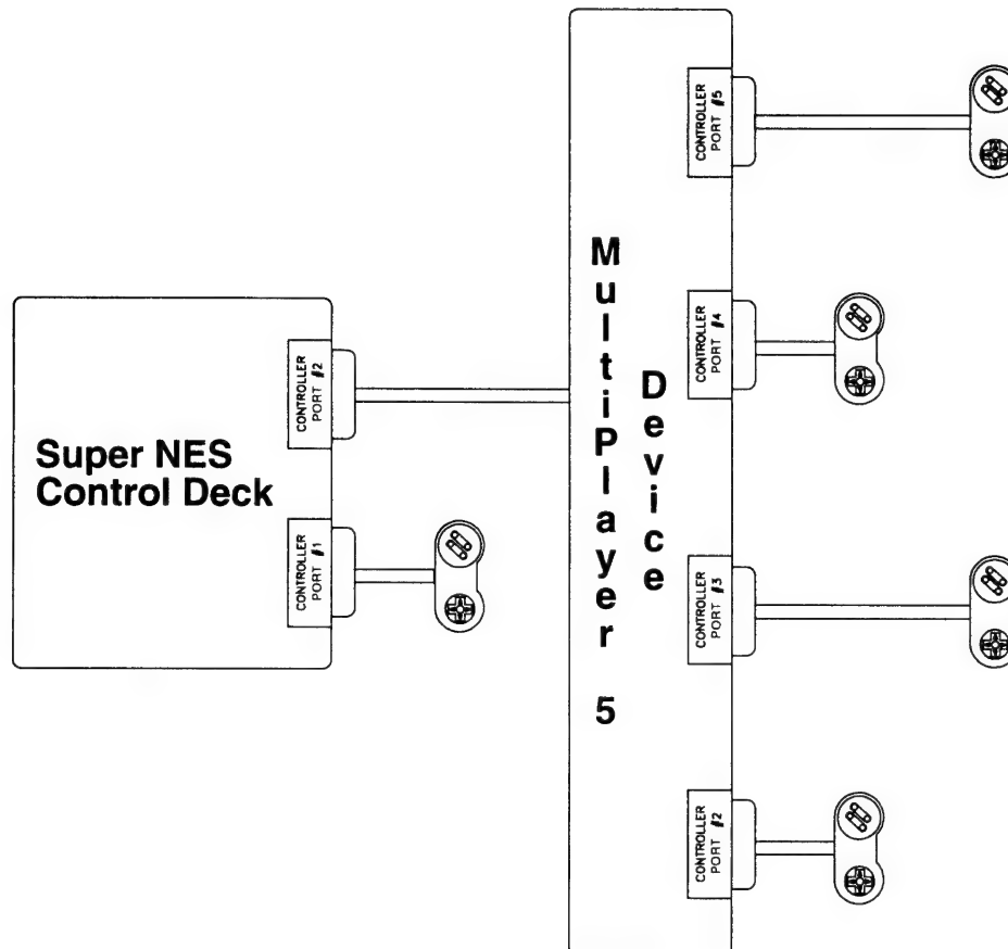
Figure 4-9-1 MultiPlayer 5 Device Hardware Connections
