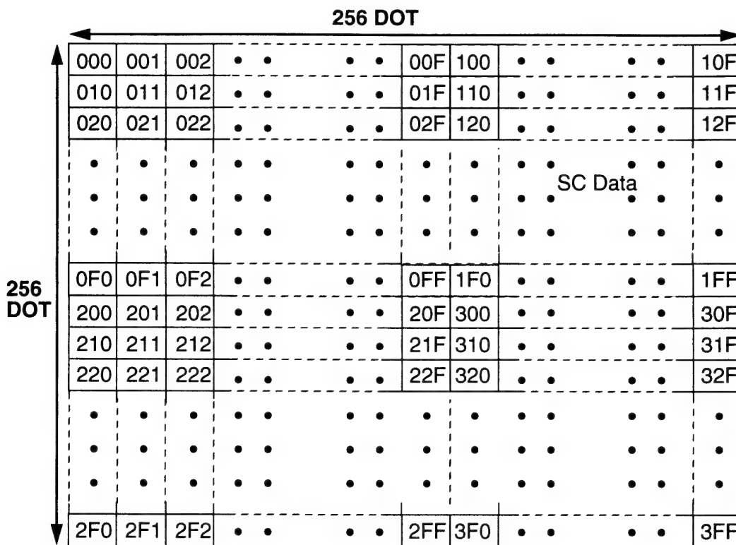
Figure 2-8-4 OBJ Character Array (numbers are hexadecimal)
