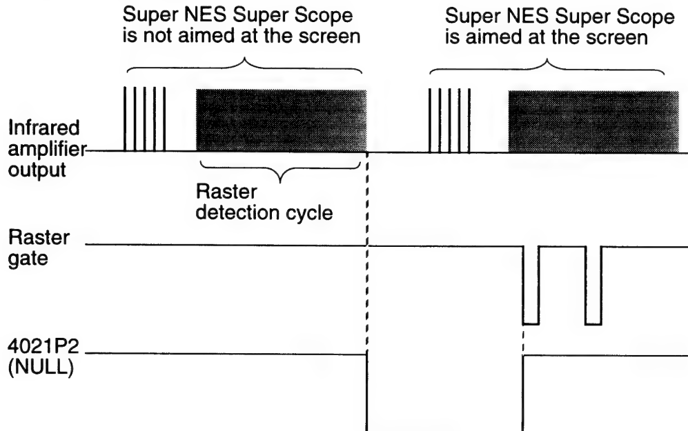
Figure 4-4-9 Null Bit
