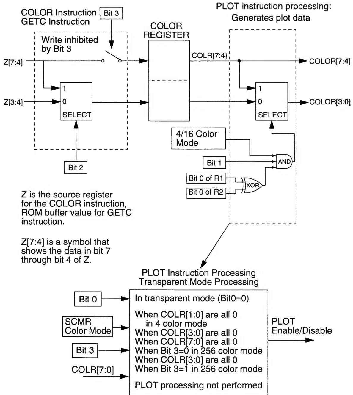
Figure 2-8-5 Plot Operations Assigned by CMODE
