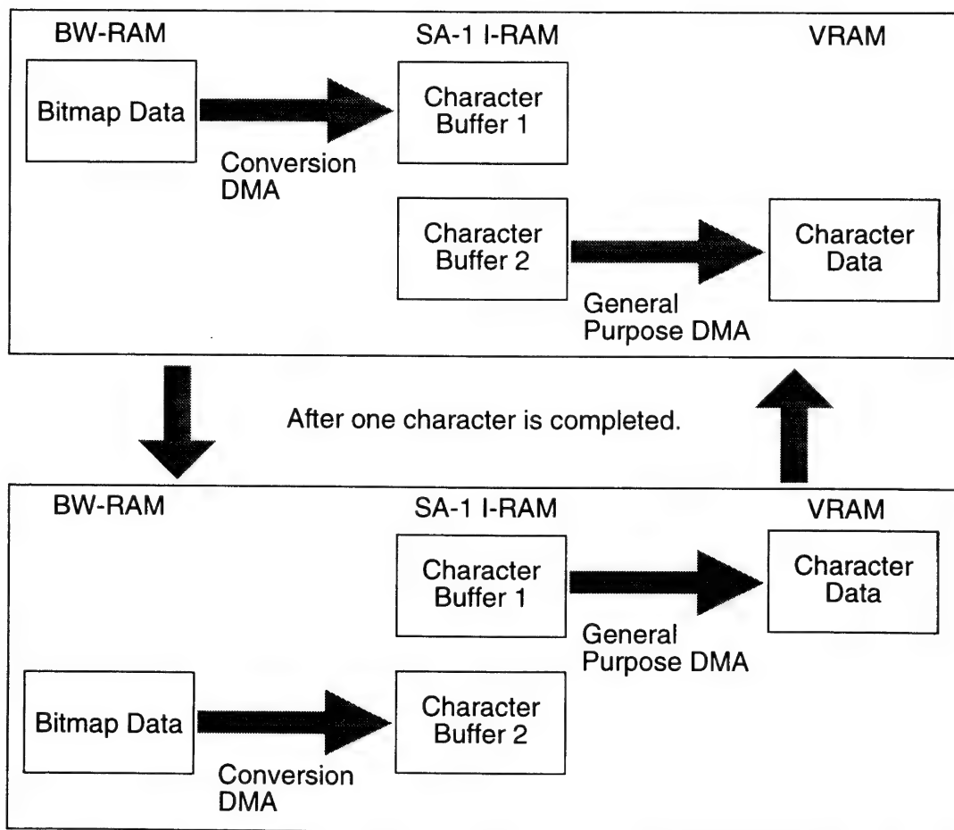
Figure 1-6-7 Character Conversion Buffers
