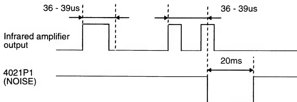
Figure 4-4-8 Noise Flag
