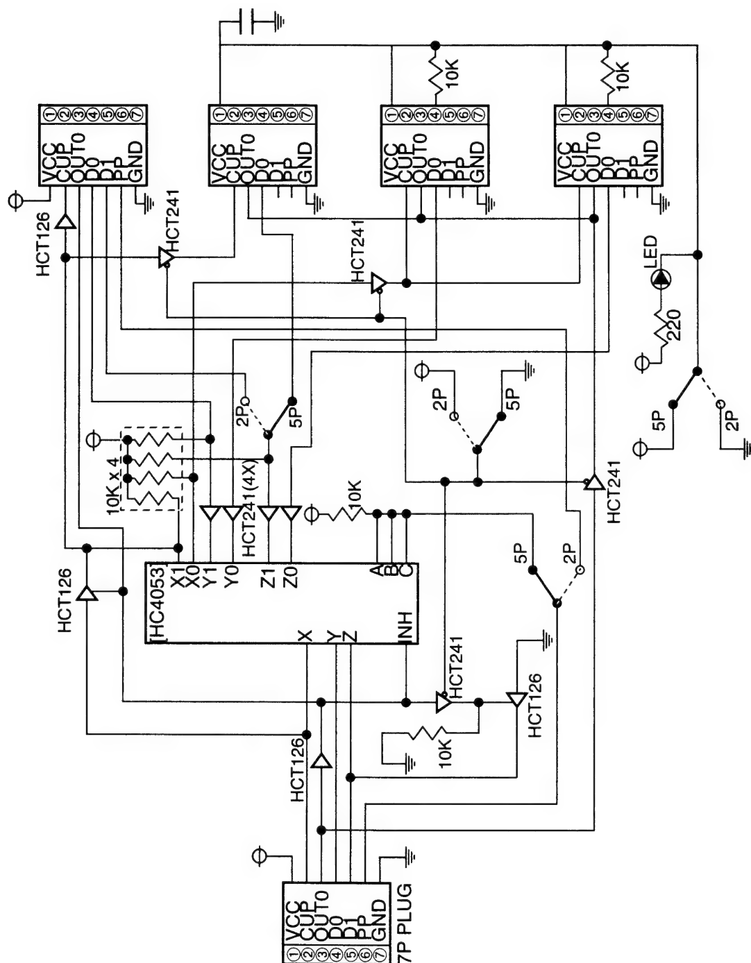
SUPER NES MultiPlayer 5 - SCHEMATIC DIAGRAM (Rev 2.3) May 1, 1992
