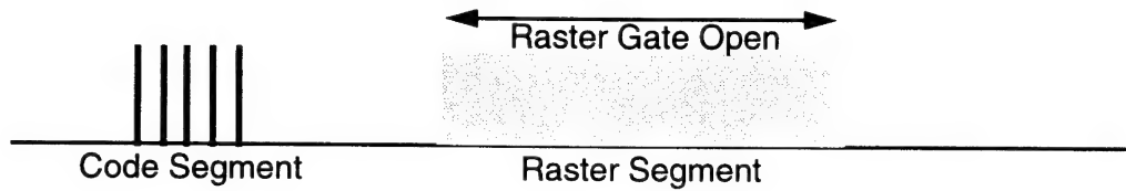
Figure 4-3-3 Raster Signal
