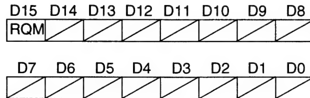
Figure 3-4-2 DSP1 Status Register Configuration
