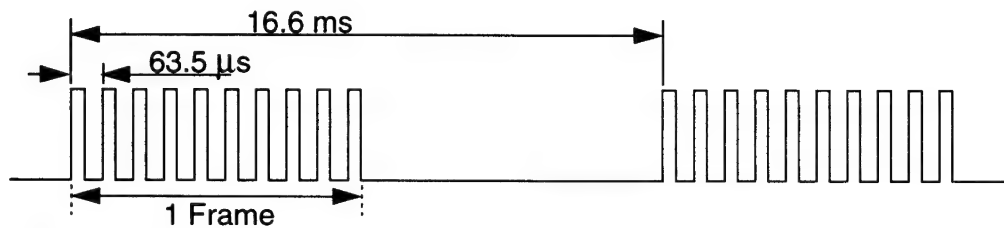
Figure 4-2-4 Vertical Positioning
