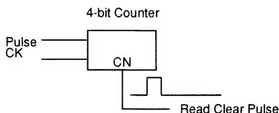
Upper Level 4-bit Counter Timing
